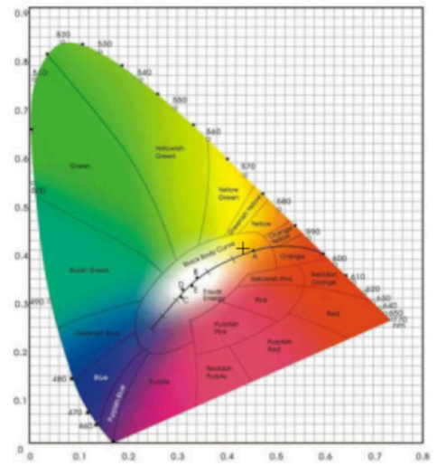
CIE1931
